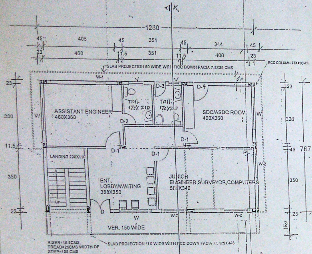
PLAN AT LEVEL-1 FLOOR
