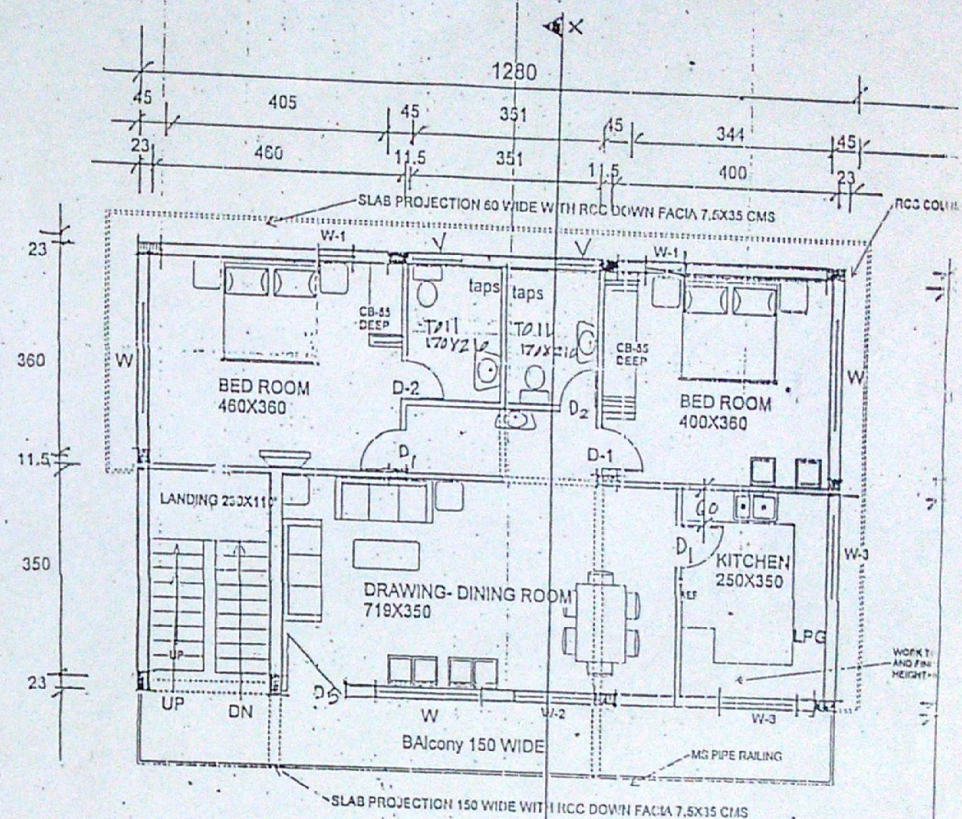
PLAN AT LEVEL-2 FLOOR
